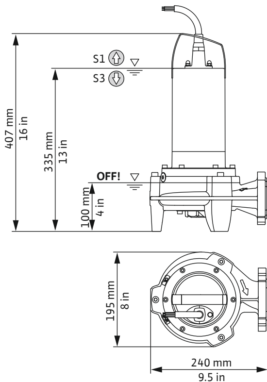
Fig. 3: Installation dimensions
