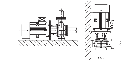
Fig. 15: CronoBloc-BL-E
